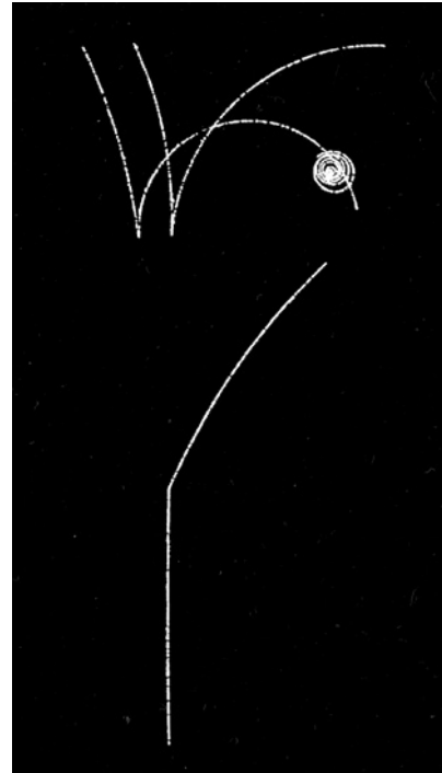
A negative kaon ( K^- ) enters a bubble chamber from the bottom and decays into a \pi^- , which moves off to the right, and a \pi^0 , which immediately decays into two photons, whose paths are indicated by the dashed lines in the drawing. Each photon interacts in the lead sheet, producing an electron-positron pair. The spiral at the right is an electron that has been knocked out of an atom in the chamber. (Other, extraneous tracks have been removed from the photograph.)
