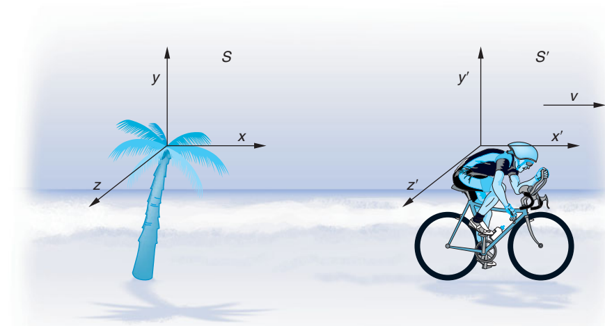
Figure 1-1 Inertial reference frame S is attached to Earth (the palm tree) and S' to the cyclist. The corresponding axes of the frames are parallel, and S' moves at speed v in the +x direction of S .
